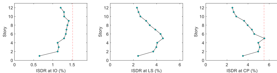
Figure 5. ISDR profiles of the optimal design II at seismic performance levels obtained through nonlinear response history analysis
