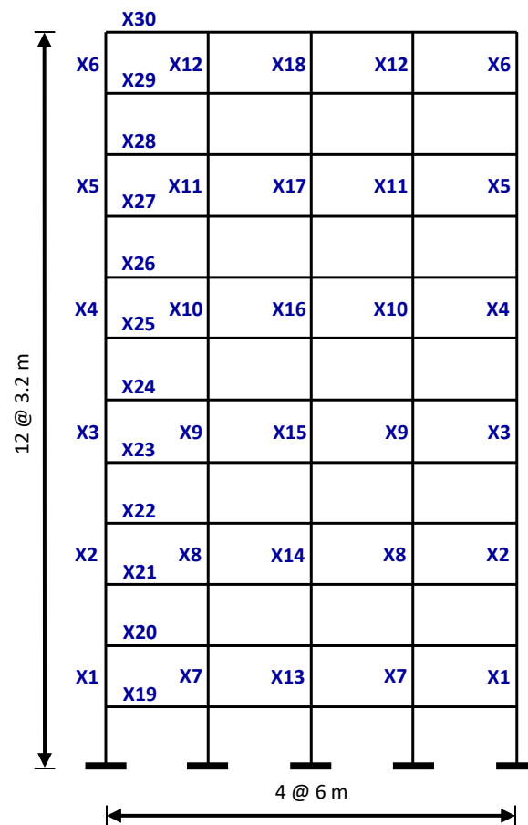
Figure 2. 12-story steel moment frame
