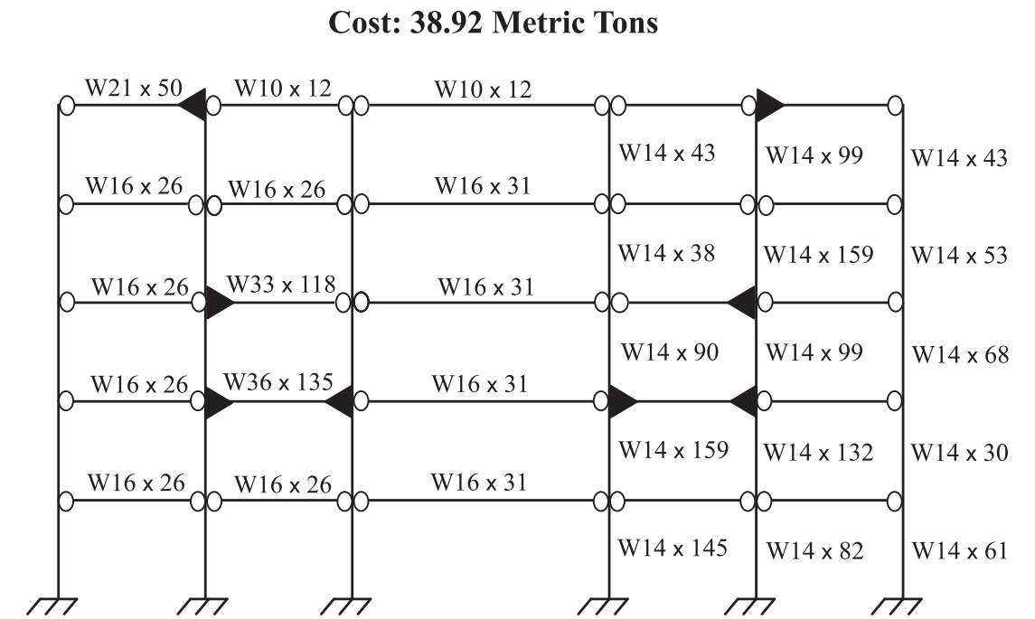
Figure 20. Best 5×5 designs from binary genetic algorithm with variable connection topology in two pools by including constraints
