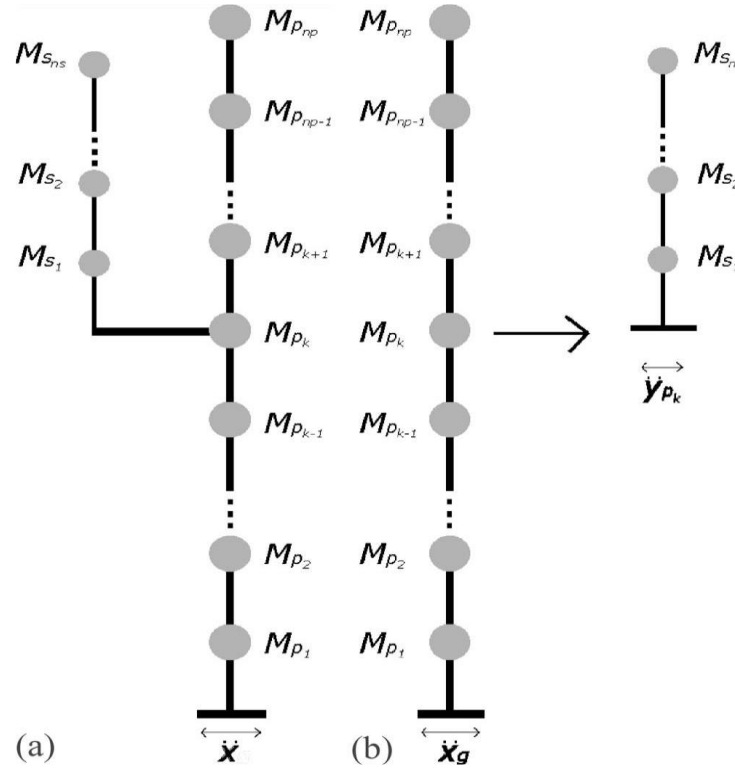
Figure 1. (a) Coupled; (b) decoupled methods [9]
