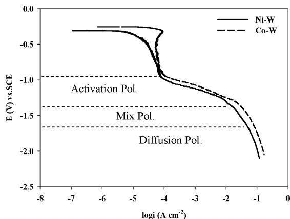
Fig. 1. Cathodic polarization plots of Ni-W and Co-W depositions obtained at room temperature (scan rate = 40 mV s -1 )
